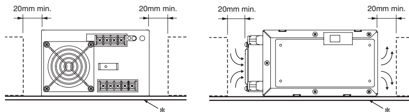
Bottom-mounting
