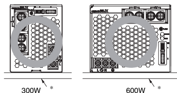
Front-mounting
