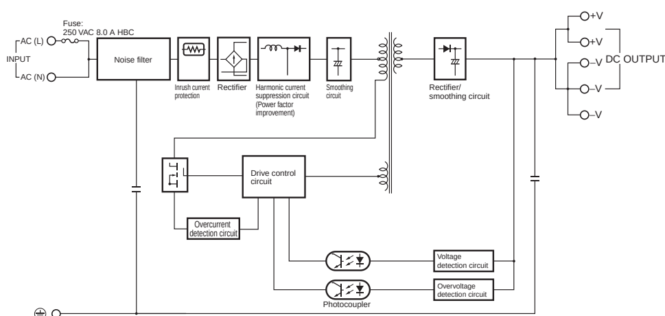
S8VK-C24024 (240W)
