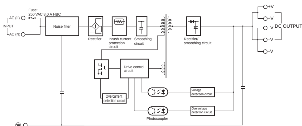
S8VK-C12024 (120W)
