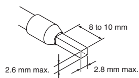
AWG24 to 12
