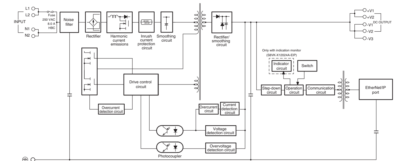
S8VK-X12024-EIP
