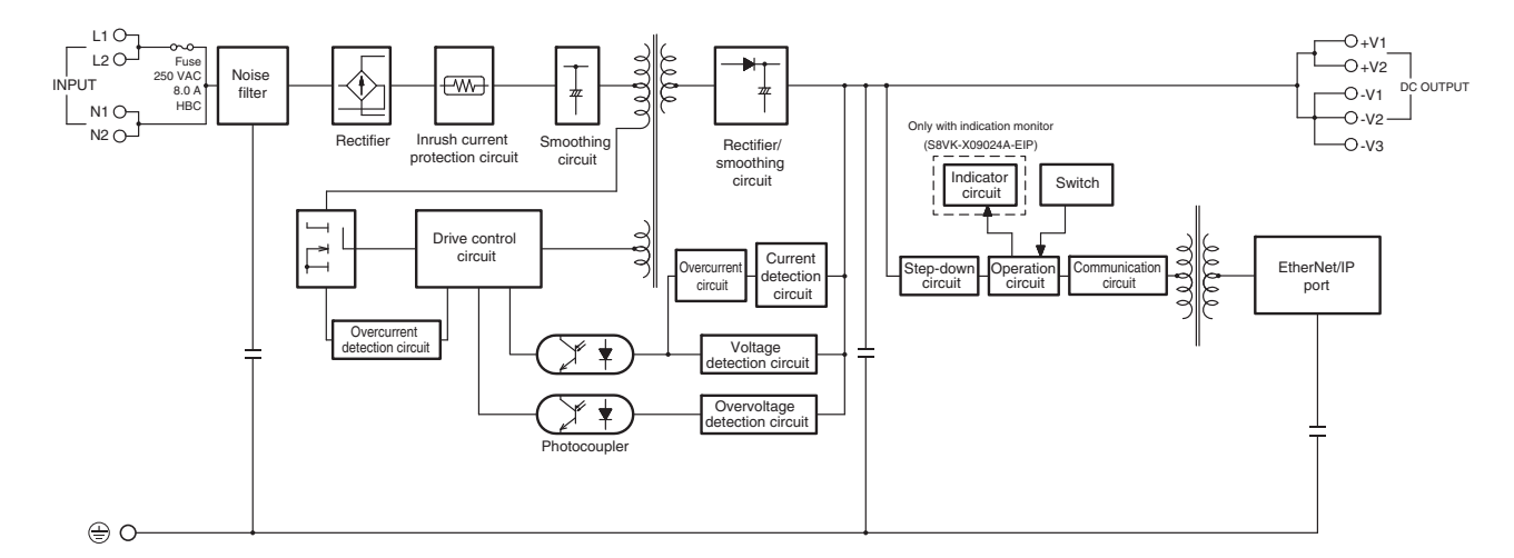
S8VK-X12024-EIP
