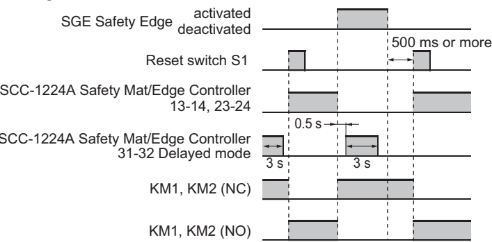
Timing Chart
