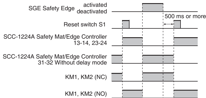
Timing Chart
