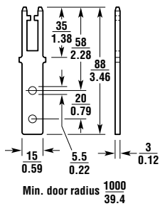
Overtravel Flat Actuator
