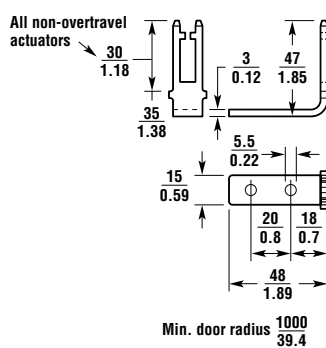
Overtravel 90-Degree Actuator
