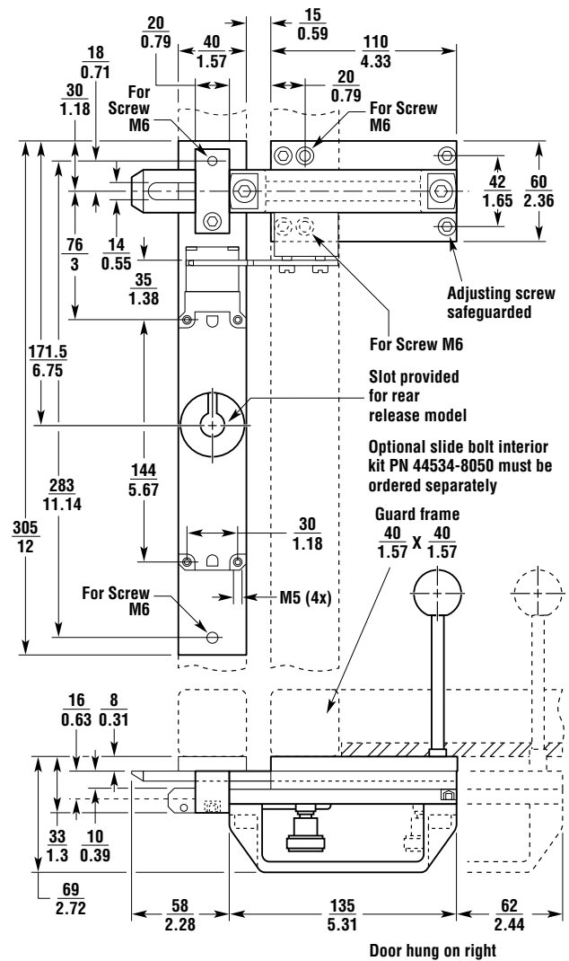
Optional Metal Slide Bolt for TL4019
