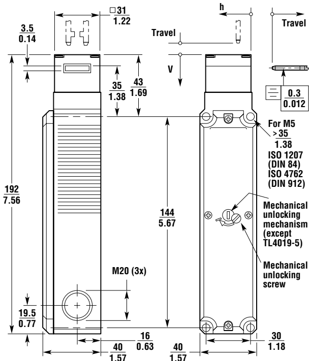
Overtravel Flat Actuator
