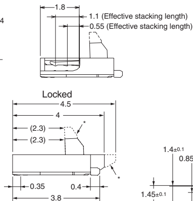
Cross-section diagram :X-X
