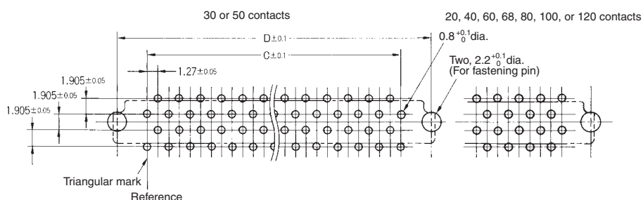
Mounting holes (bottom view)
