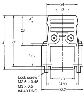
15, 25 and 37-contact Hood with Straight Connecting Cable XM2S-□□1□
