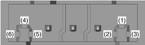
XW4M (Plug, Single-Row Type)
