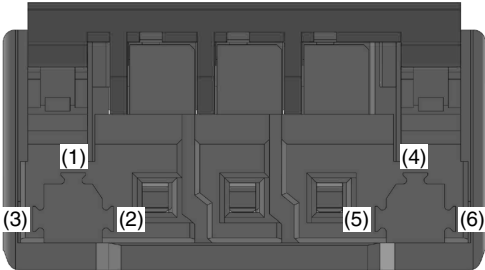
XW4N (Socket, Double-Row Type)
