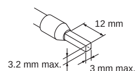
Ferrule Processed Dimensions
