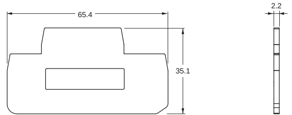
XW5E-P2.5-1.2-1
