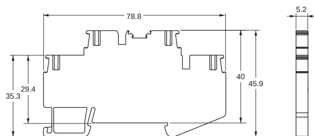
XW5T-P2.5-1.1-2 (BL)/XW5G-P2.5-1.1-2
