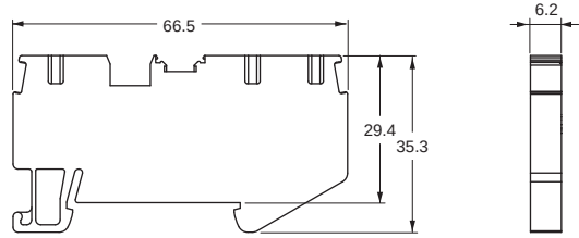
XW5T-P4.0-1.1-2 (BL)/XW5G-P4.0-1.1-2
