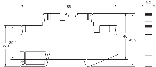
XW5T-P4.0-1.1-2 (BL)/XW5G-P4.0-1.1-2
