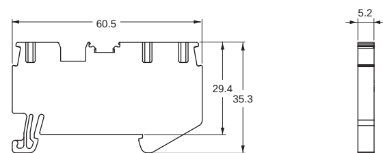
XW5T-P2.5-1.2-1 (BL)/XW5G-P2.5-1.2-1
