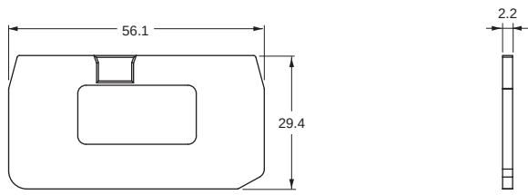
XW5E-P4.0-2.2-1
