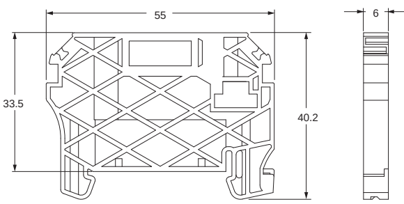
XW5Z-EP6 (End Brackets)
