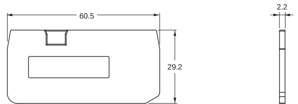
XW5E-P2.5-1.1-2
