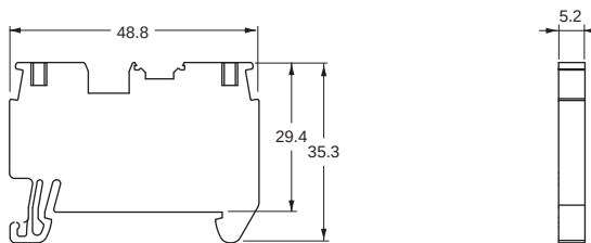
XW5T-P2.5-1.1-1 (BL)/XW5G-P2.5-1.1-1
