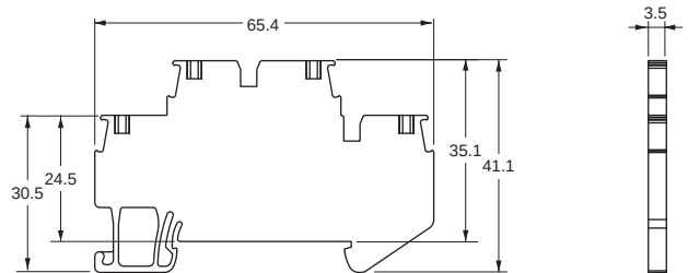
XW5T-P2.5-1.2-1 (BL)/XW5G-P2.5-1.2-1
