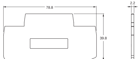
XW5E-P2.5-1.1-2
