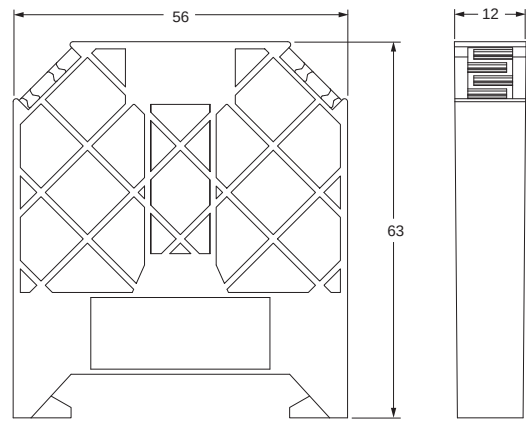
XW5Z-EP12 (Separator Plates)
