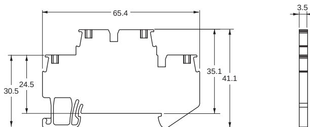
XW5T-P2.5-1.2-1 (BL)/XW5G-P2.5-1.2-1
