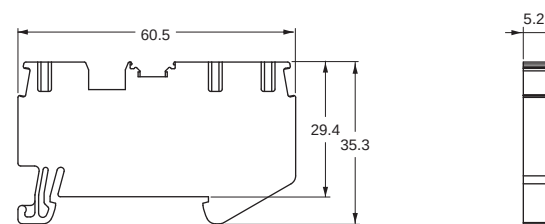
XW5T-P2.5-1.2-1 (BL)/XW5G-P2.5-1.2-1
