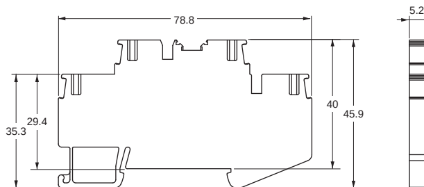
XW5T-P2.5-1.1-2 (BL)/XW5G-P2.5-1.1-2
