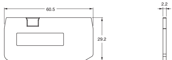
XW5E-P2.5-1.1-2
