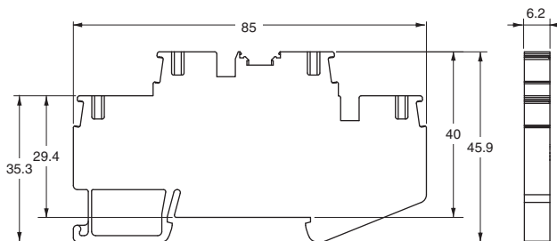
XW5T-P4.0-1.1-2 (BL)/XW5G-P4.0-1.1-2
