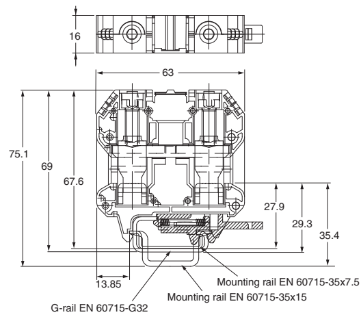
XW5G-S35-1.1-1
