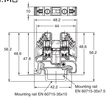
XW5T-S35-1.1-1□
