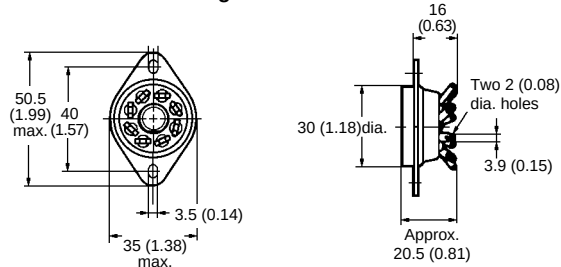
P3G-08 Back mounting socket
