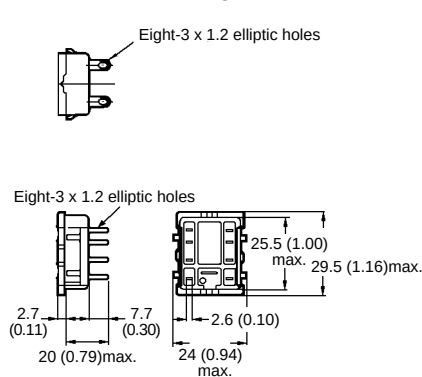
PY08 Panel mounting socket
