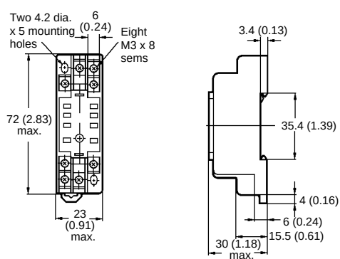
PYF08A-E Bottom surface or track mounting socket
